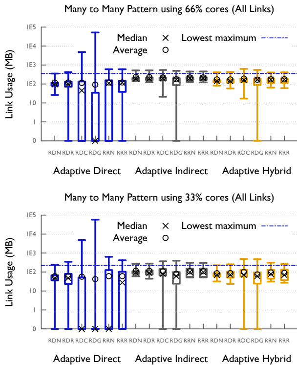
Fig. 8: Traffic distribution for M2M on 66% and 33% cores.
